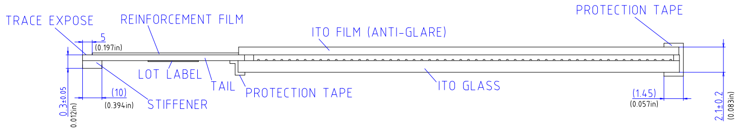
SECTION A
