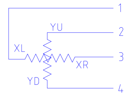
PIN ASSIGNMENT
