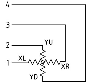
Pin Assignment
