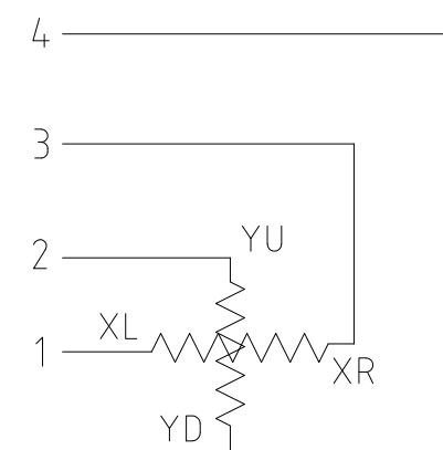
Pin Assignment
